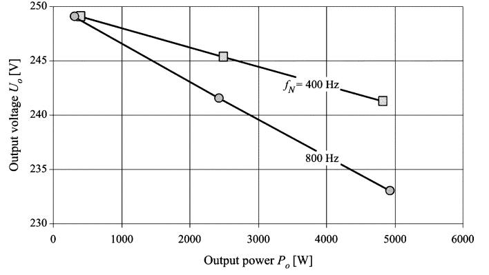
Fig. 3. Dependency of the rectifier output voltage on the output power for U_{N,rms} = 115 V and mains frequencies f_N = 400 Hz, 800 Hz as determined by digital simulation. Simulation parameters: see Table I, coupling of the windings of a phase leg of the inpterphase transformer assumed ideal.
