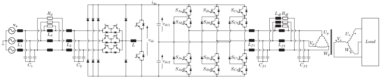
Fig. 1. Scheme of the developed ground power unit for aircraft applications.
